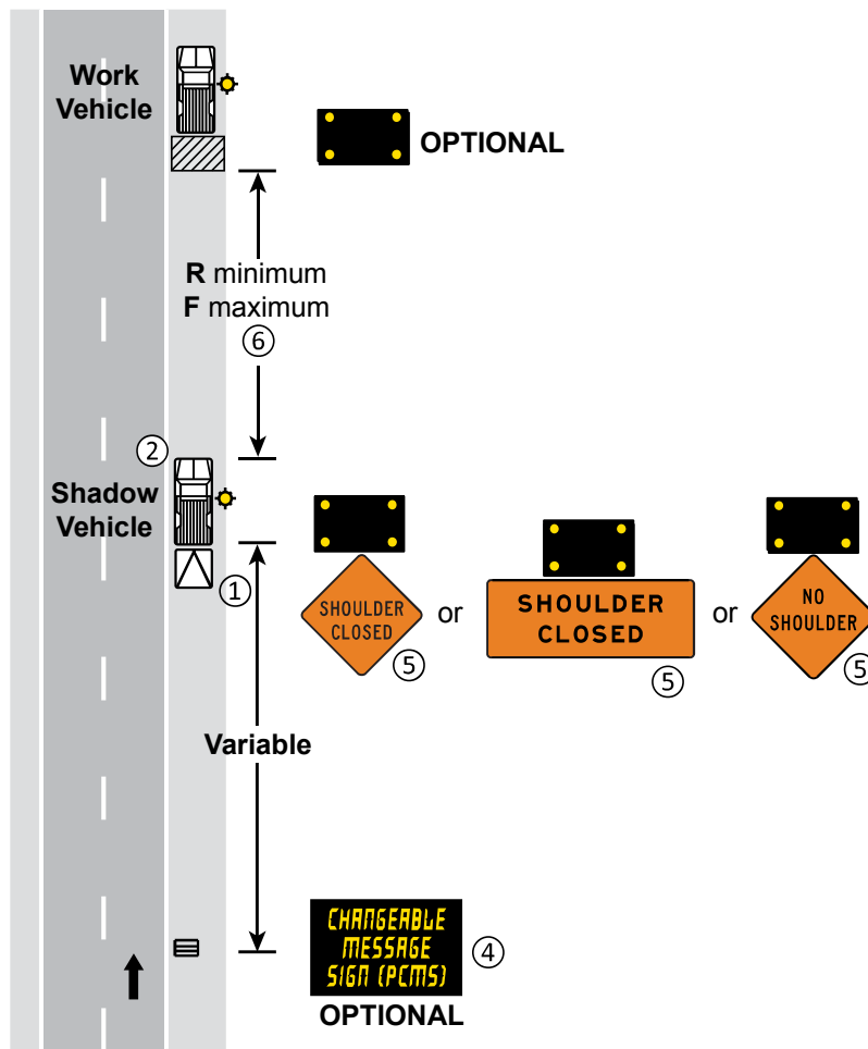
1 HOUR or LESS SHOULDER CLOSURE Mobile and Short Duration LAYOUT 9 6K-9
