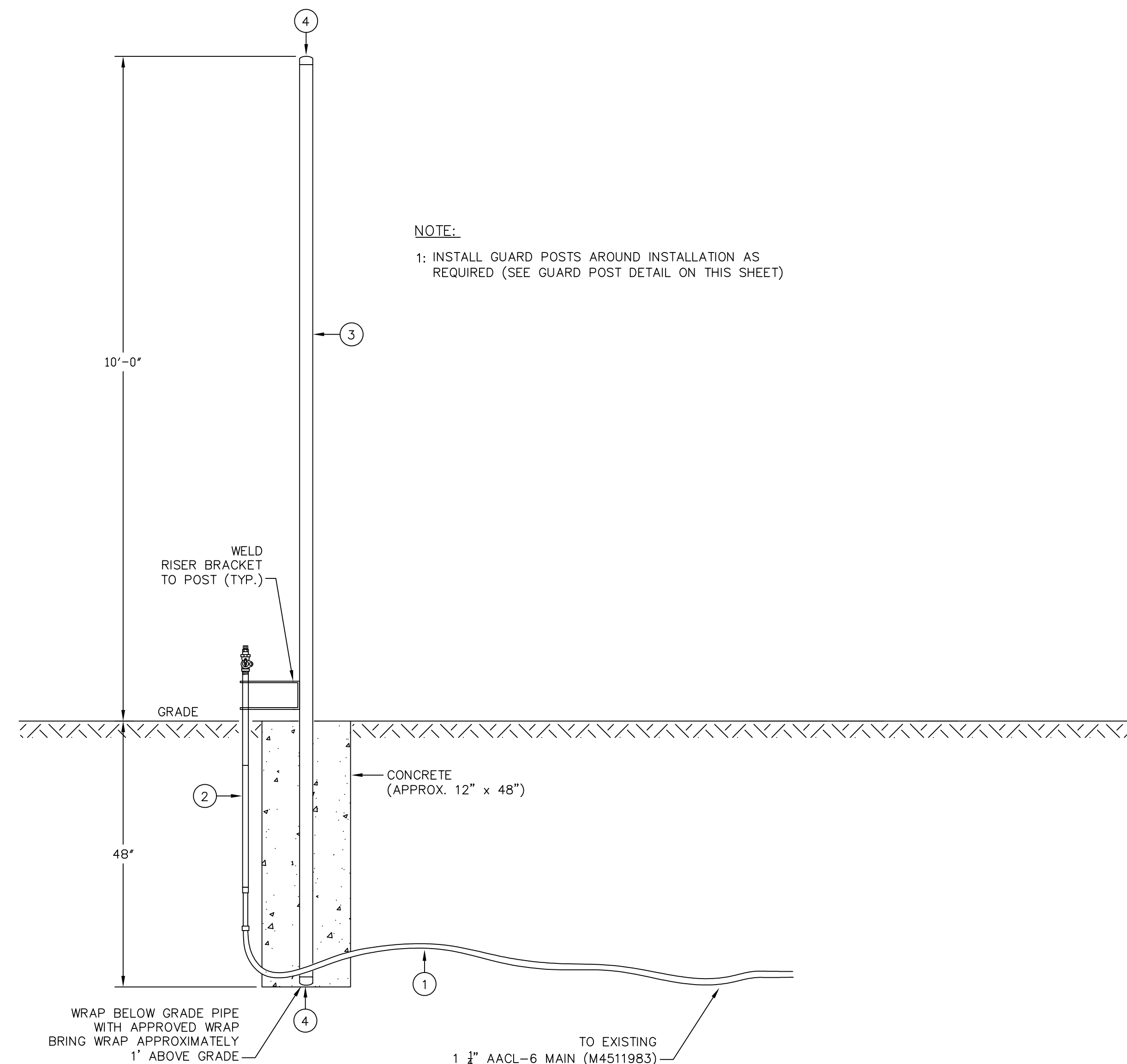
TELEMETERING DETAIL SCALE: 3/4" = 1'-0"
